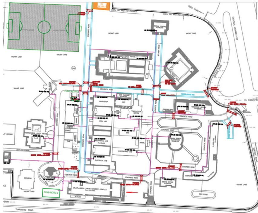
LAYOUT PLAN
